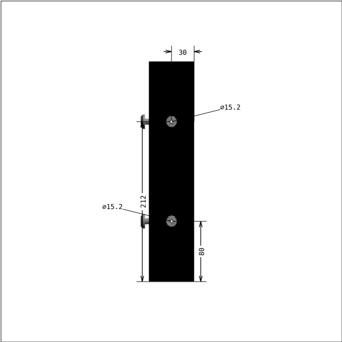
DRAWING 6, Pos 7 SIDE 1, bar length: 292.0 mm
