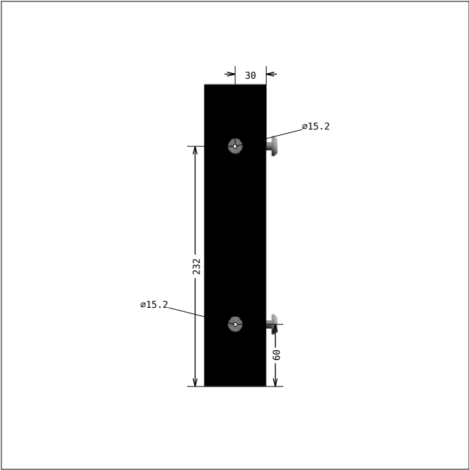
DRAWING 12, Pos 14 SIDE 3
