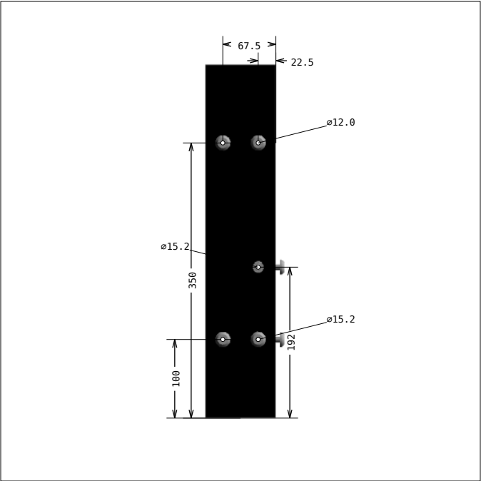
DRAWING 10, Pos 11 SIDE 2
