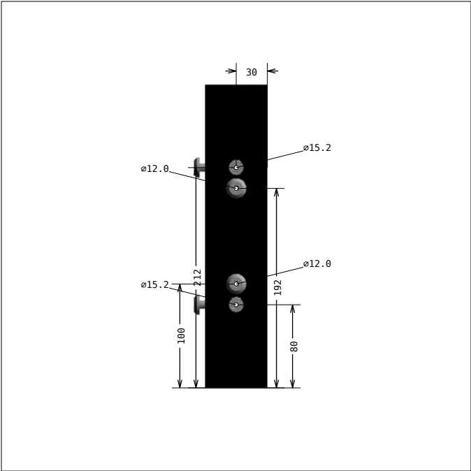
DRAWING 7, Pos 8 SIDE 1, bar length: 292.0 mm
