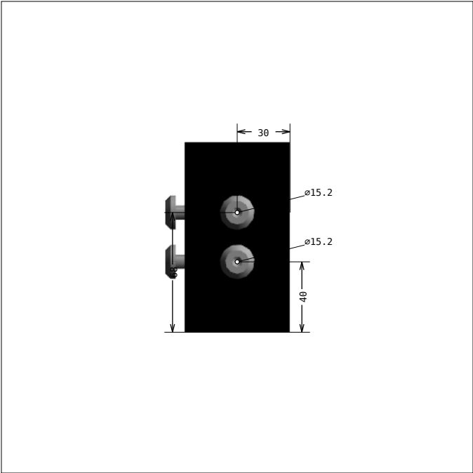
DRAWING 1, Pos 1 SIDE 1, bar length: 108.0 mm
