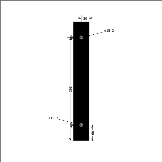
DRAWING 13, Pos 15 SIDE 1, bar length: 450.0 mm
