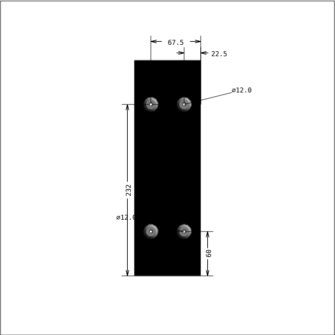
DRAWING 12, Pos 14 SIDE 2
