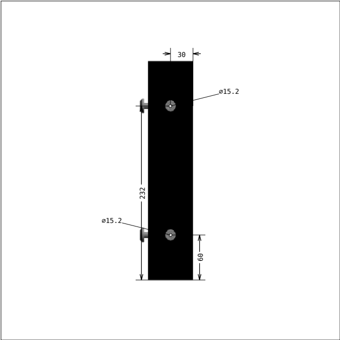
DRAWING 12, Pos 14 SIDE 1, bar length: 292.0 mm
