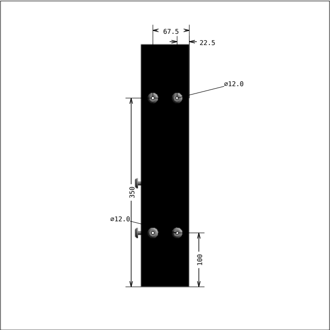
DRAWING 9, Pos 10 SIDE 2
