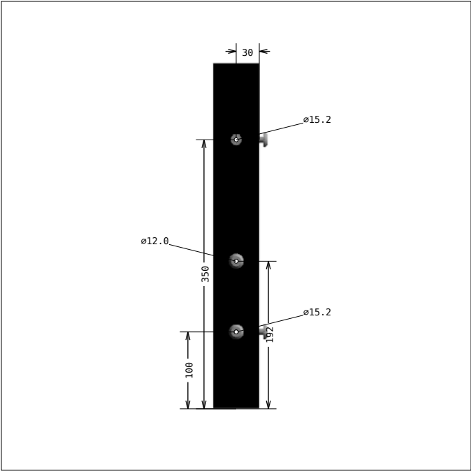
DRAWING 9, Pos 10 SIDE 3
