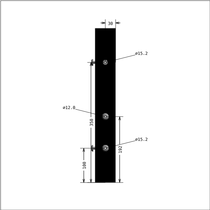
DRAWING 10, Pos 11 SIDE 1, bar length: 450.0 mm
