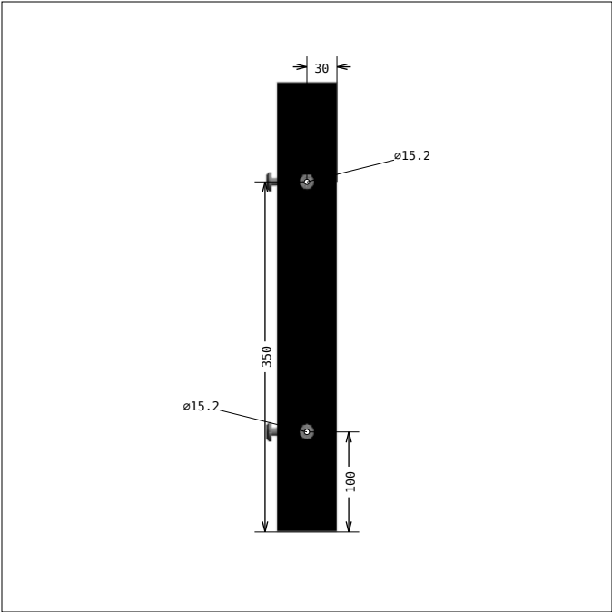
DRAWING 9, Pos 10 SIDE 1, bar length: 450.0 mm
