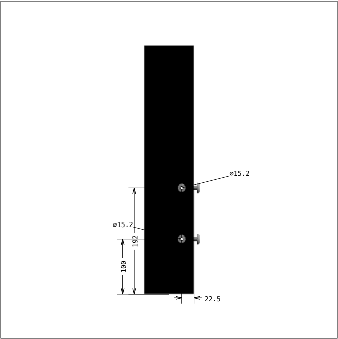
DRAWING 9, Pos 10 SIDE 4
