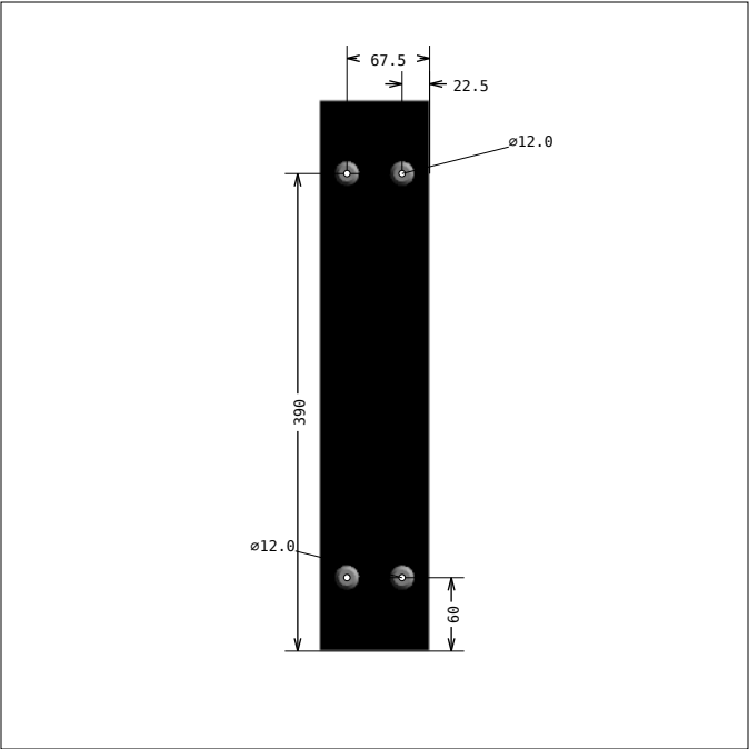
DRAWING 13, Pos 15 SIDE 2
